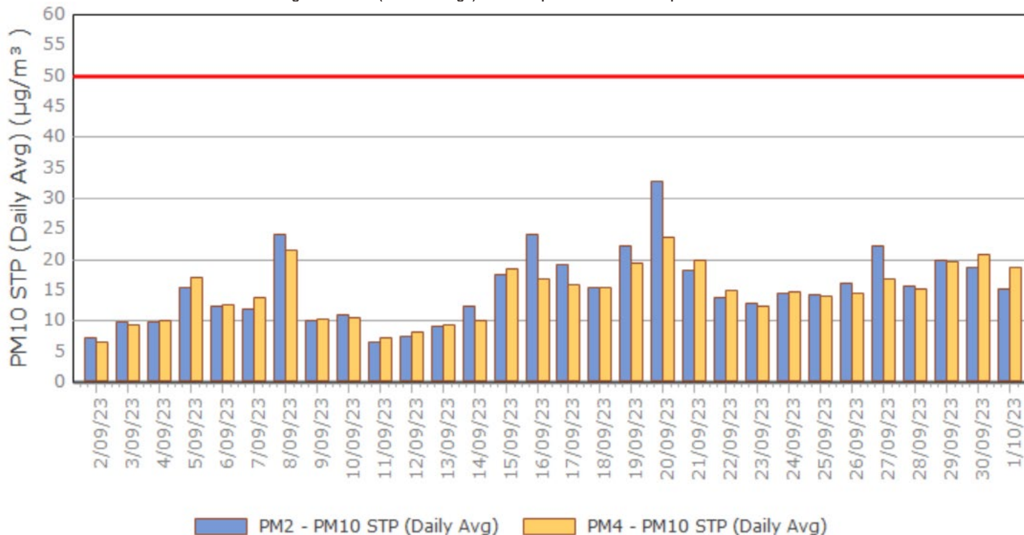
Figure 2. PM10 (24 hr Average) with Compliance Criteria – September 2023
