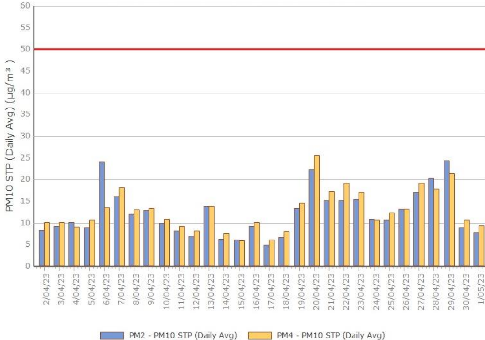
Figure 2. PM10 (24 hr Average) with Compliance Criteria – April 2023
