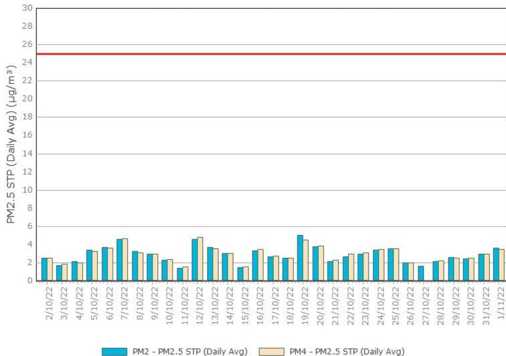
Figure 3. PM2.5 (24 hr Average) with Compliance Criteria – October 2022
