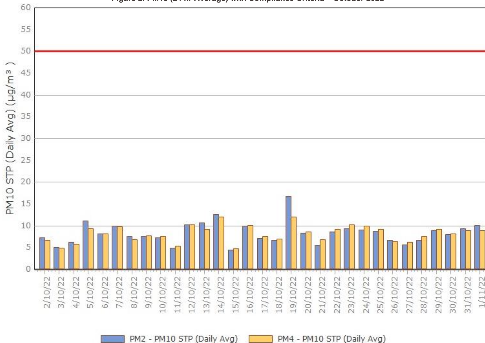
Figure 2. PM10 (24 hr Average) with Compliance Criteria – October 2022
