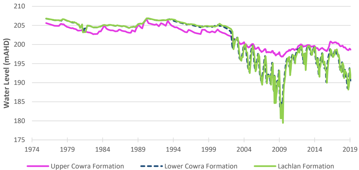
Chart 3 Hydrographs for Nested Piezometers and GW036083 and GW036526 Highlighting Millennium Drought
